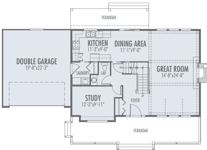
Main Floor
