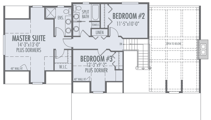
Upper Floor
