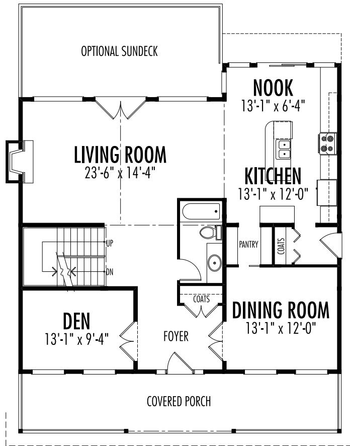
Main Floor
