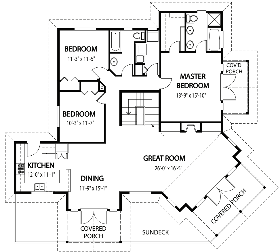
Upper Floor
