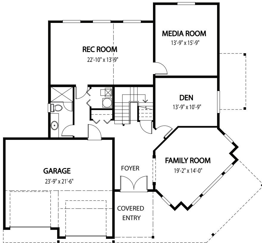
Main Floor
