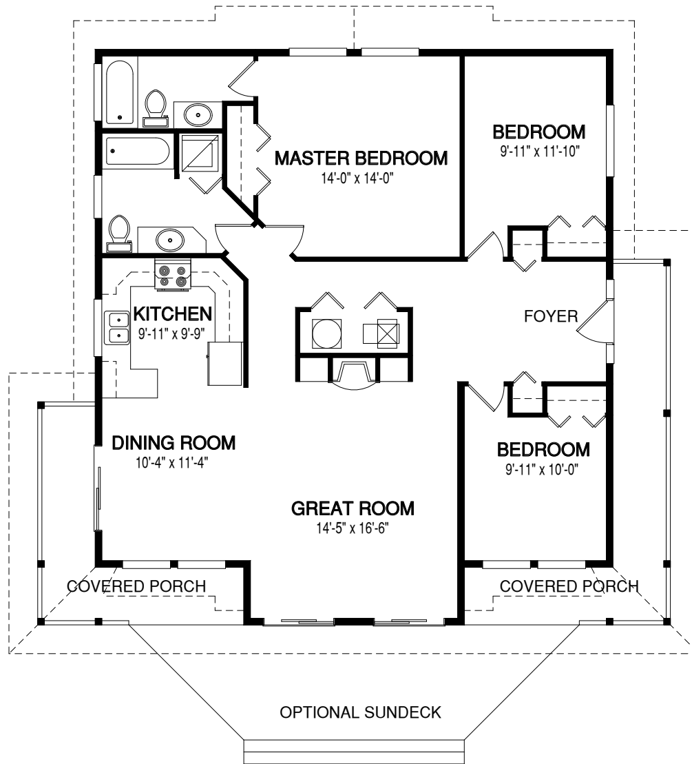
Main Floor
