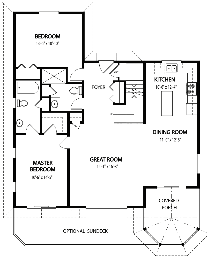
Main Floor
