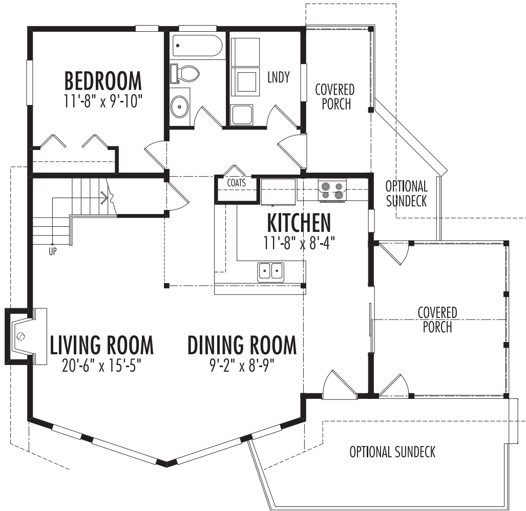
Main Floor
