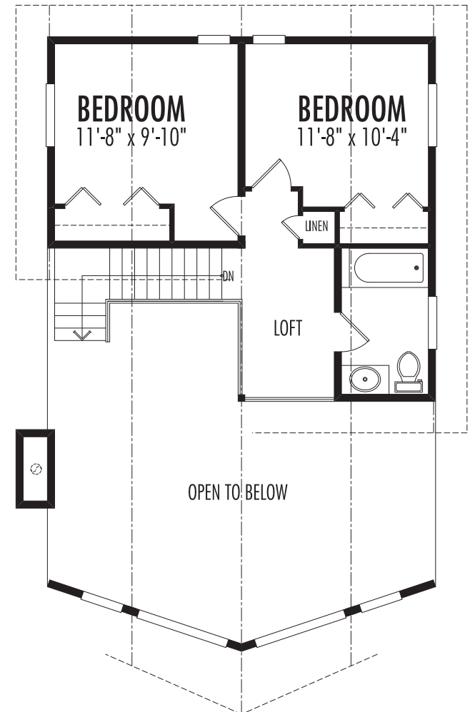
Upper Floor
