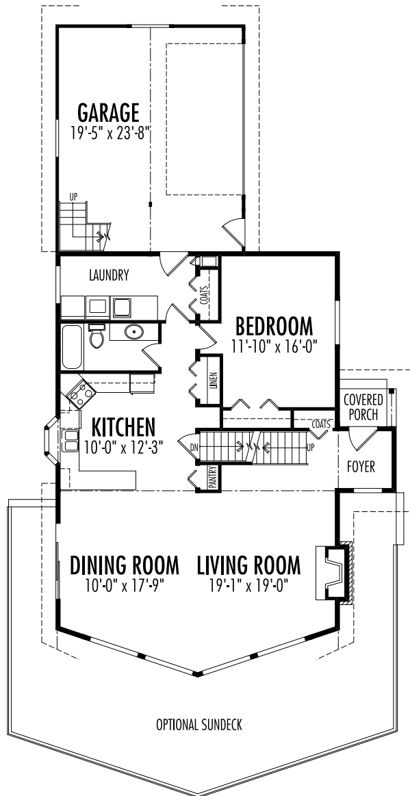
Main Floor
