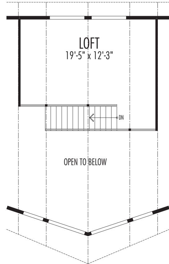
Upper Floor
