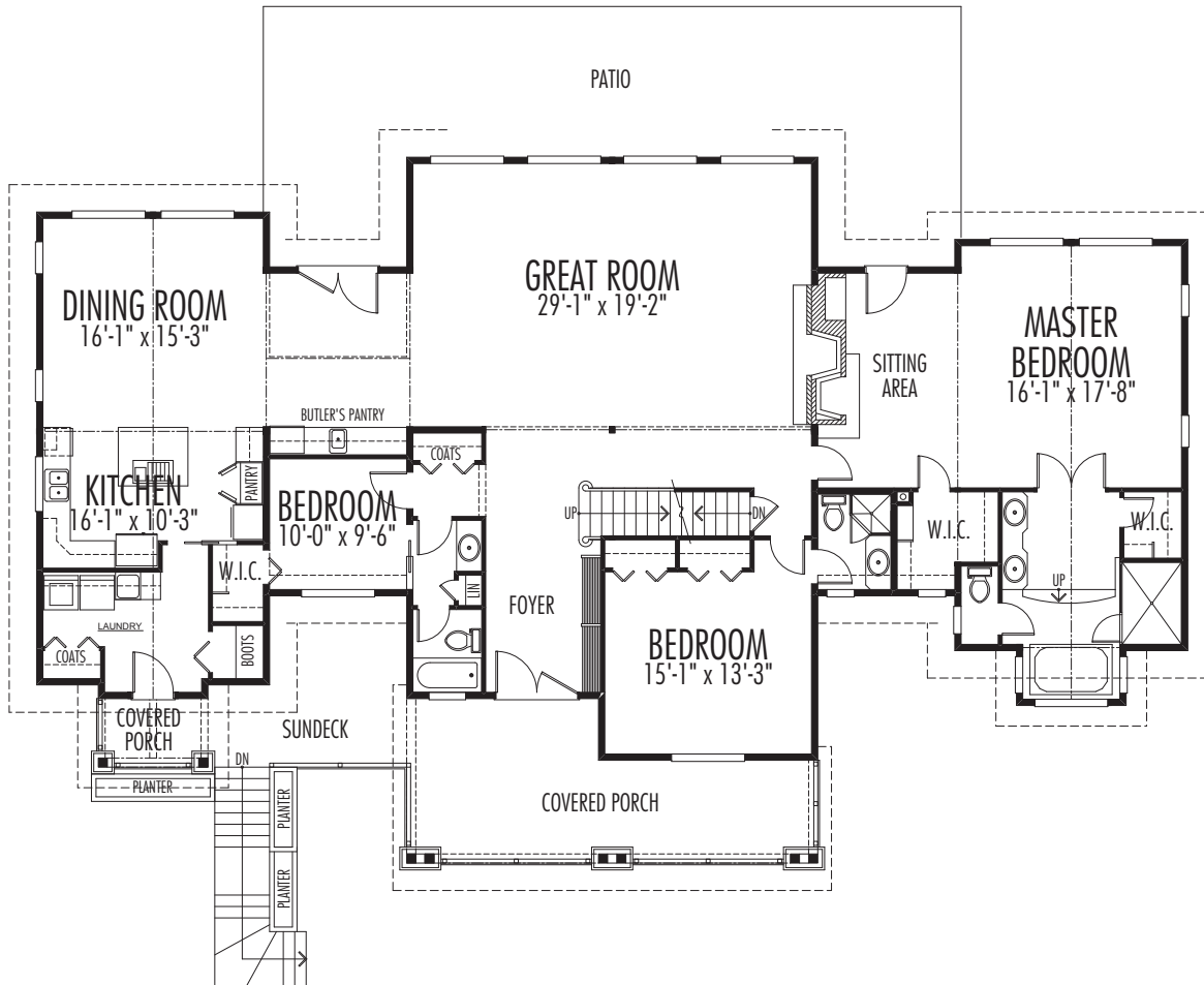
Main Floor
