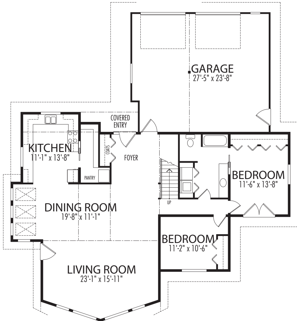
Main Floor
