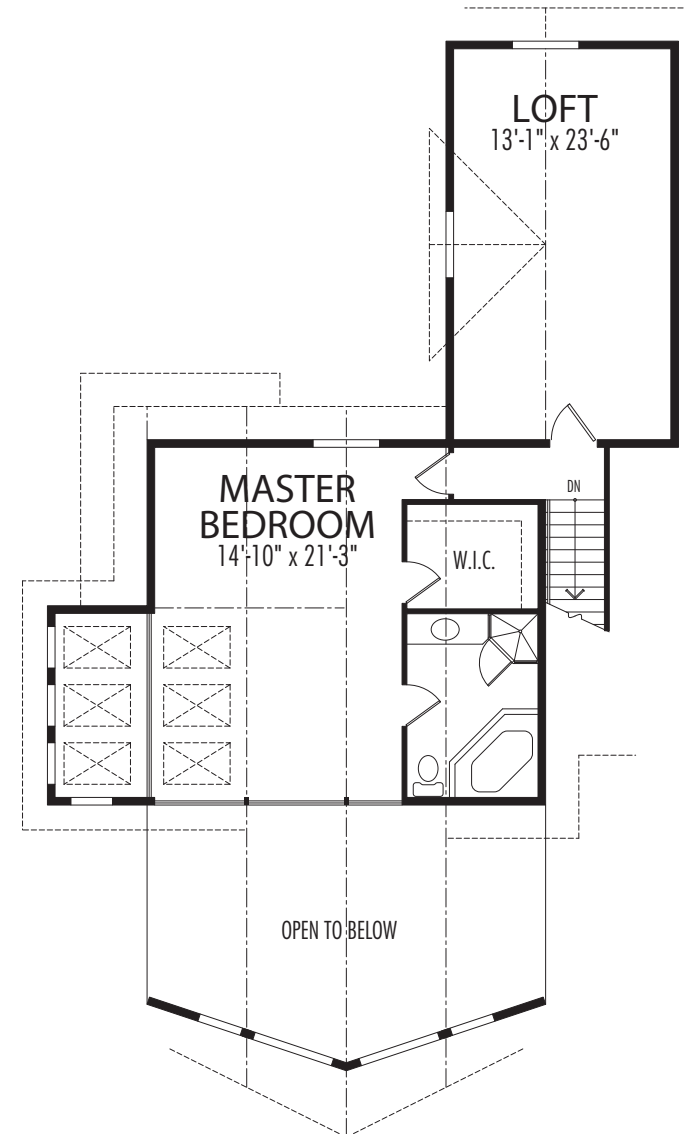
Upper Floor
