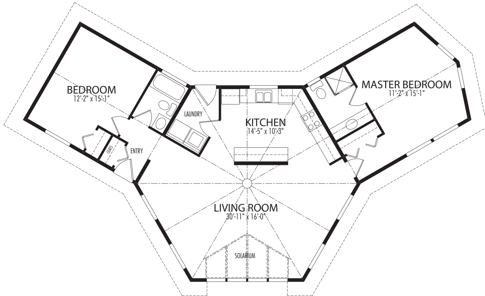
Main Floor
