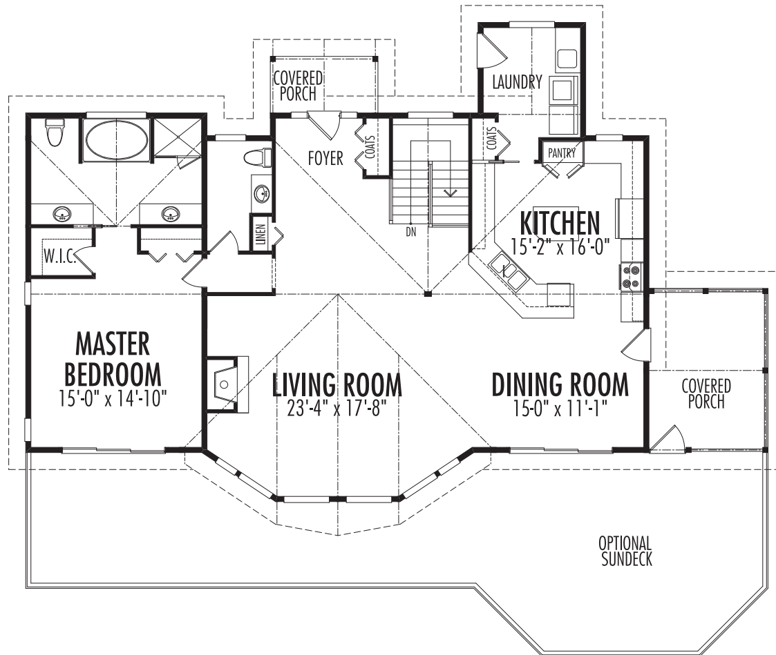
Main Floor
