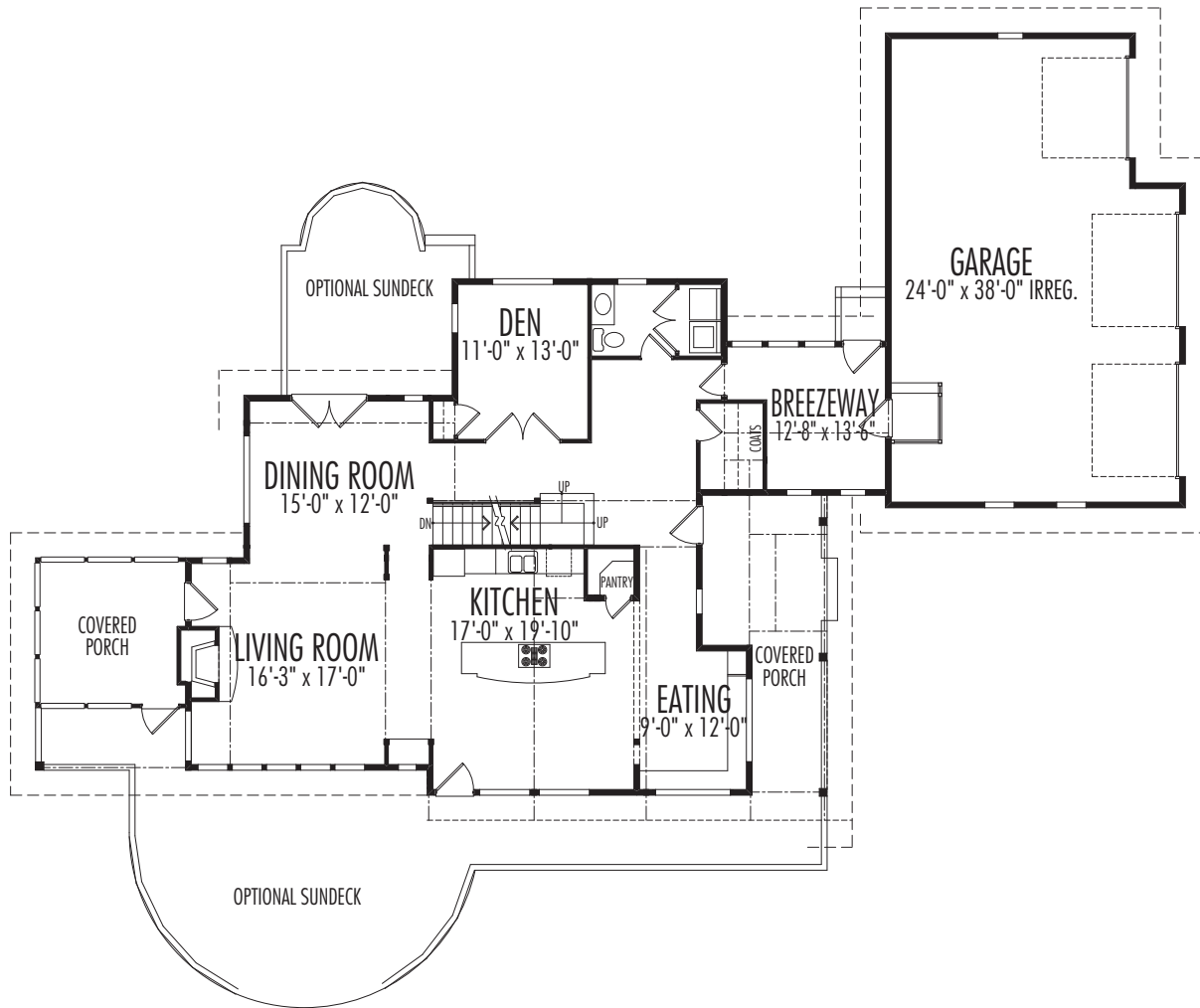
Main Floor
