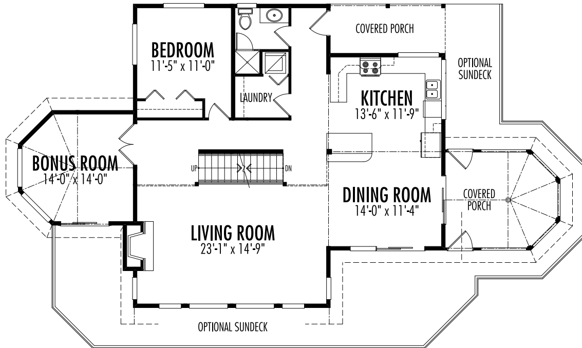
Main Floor
