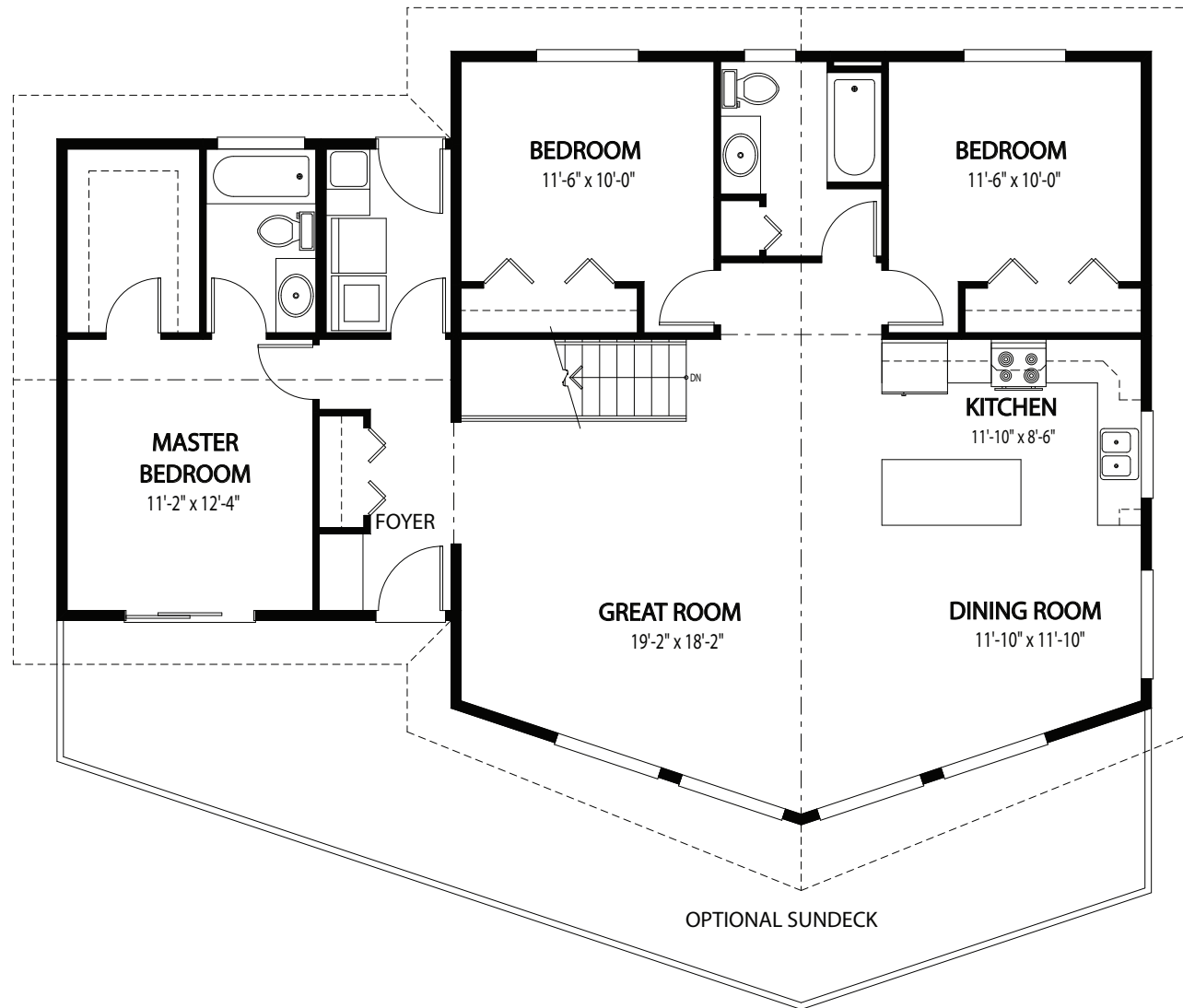
Main Floor
