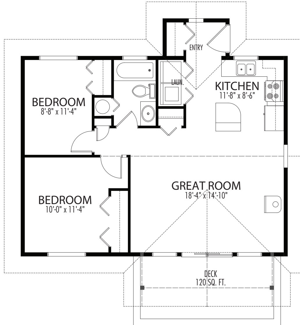
Main Floor
