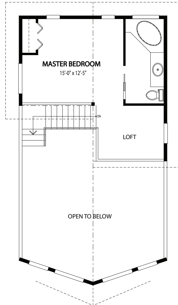
Upper Floor
