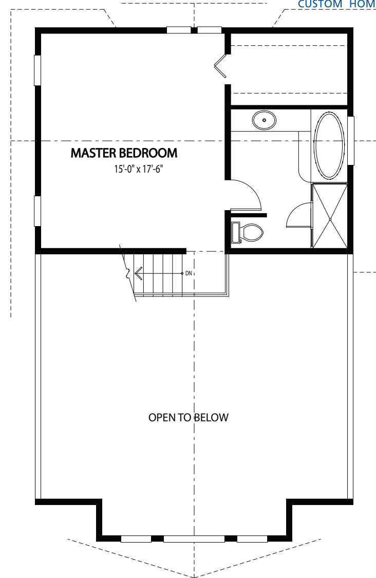
Upper Floor
