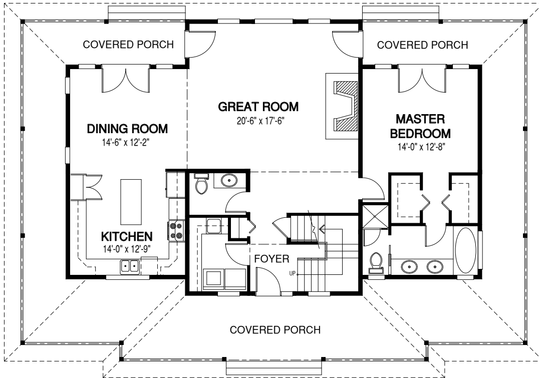
Main Floor
