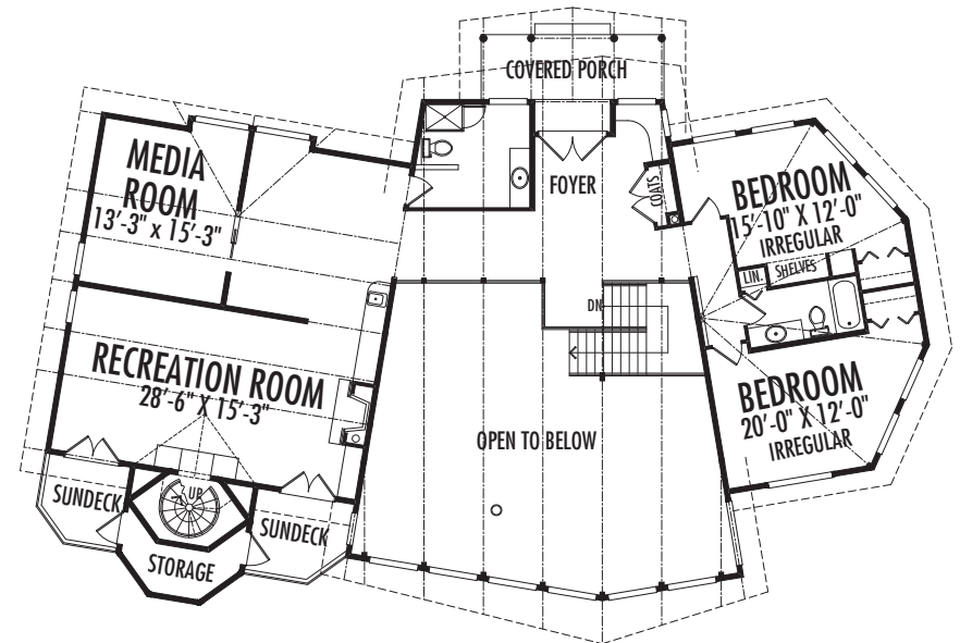
Upper Floor
