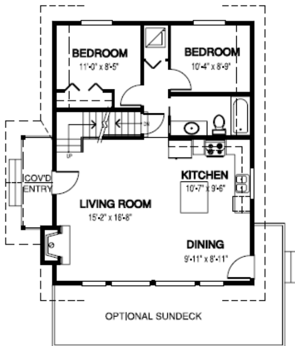
MAIN FLOOR
